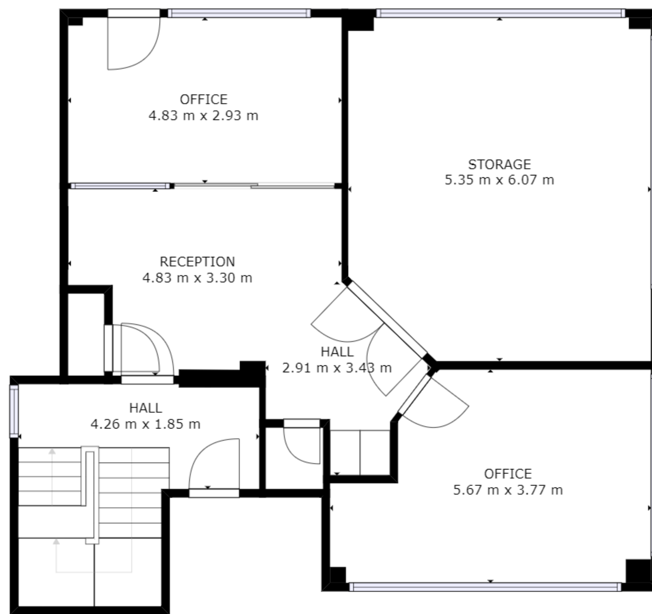
FLOOR 1
