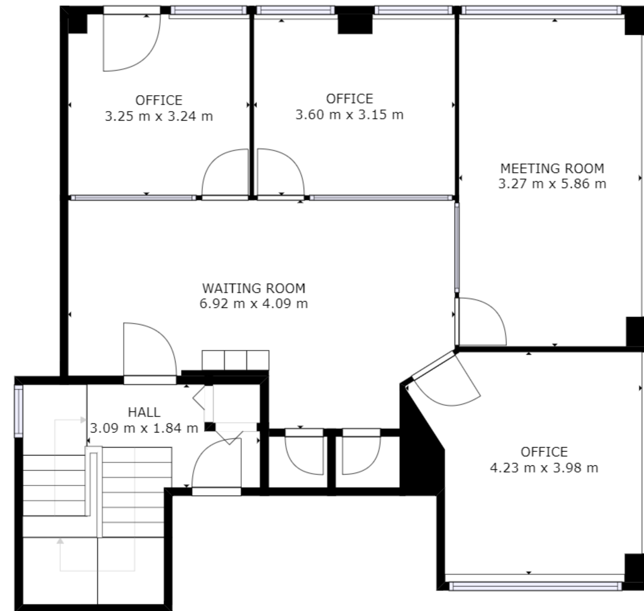
FLOOR 2
